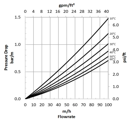
Figure 2: Pressure Drop
