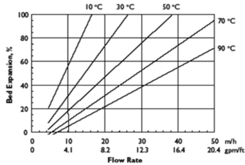
Figure 1: Backwash Expansion
