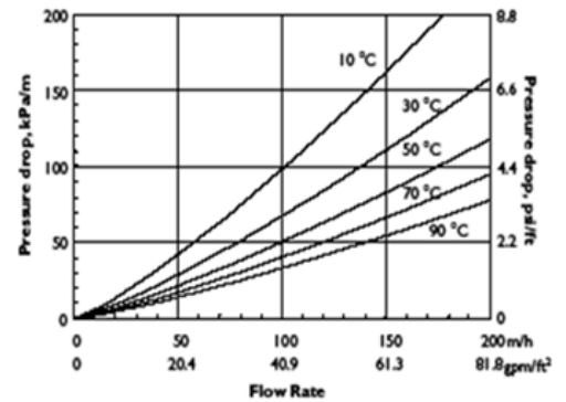
Figure 2: Pressure Drop
