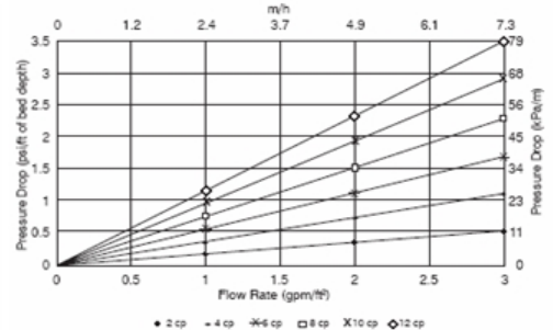
Figure 2: Pressure Drop
