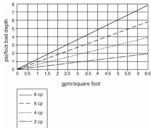
Figure 1: Pressure Drop
