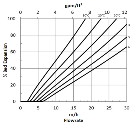
Figure 1: Backwash Expansion
